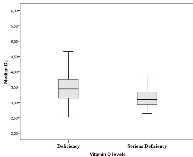
Figure 1. Box plot showing relationship between Median distal latency (DL) and Vitamin D categories.
